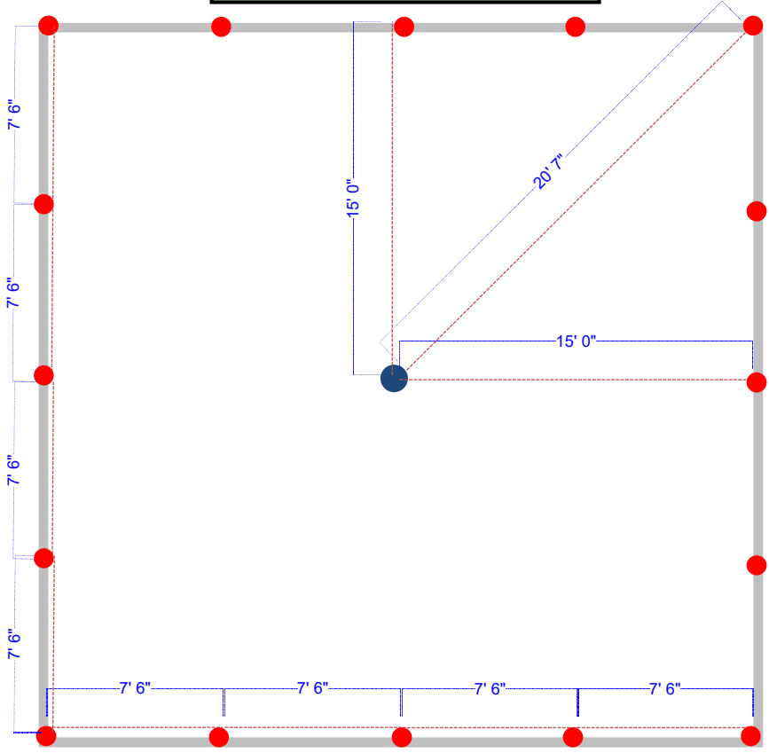
30' x 30' Pole Tent Standard & Wind - Pole placement
